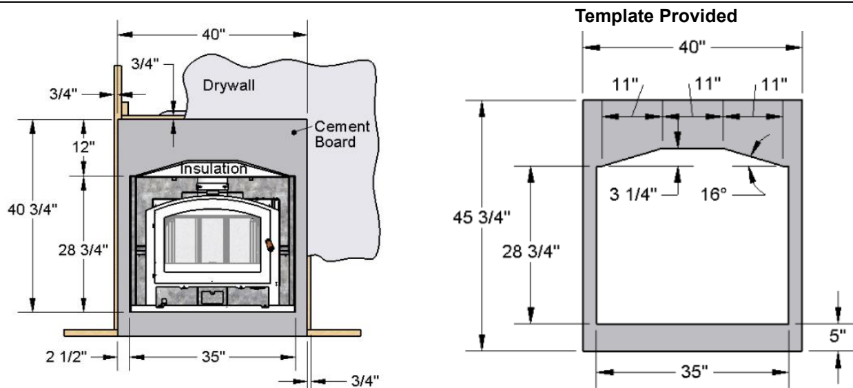
Figure 9 Minimum Requirements for Non-combustible Facing
