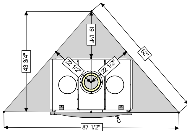
Figure 4 PEARL 3600B Framing Examples
