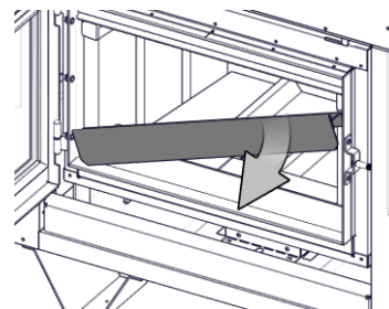
Figure 21 Ash Lip
