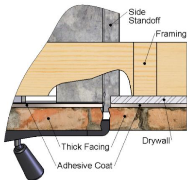
Figure 10 Framing Alignment Examples – Top Views
