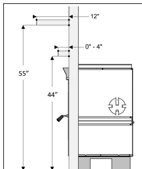
Figure 11 Mantel Requirements
