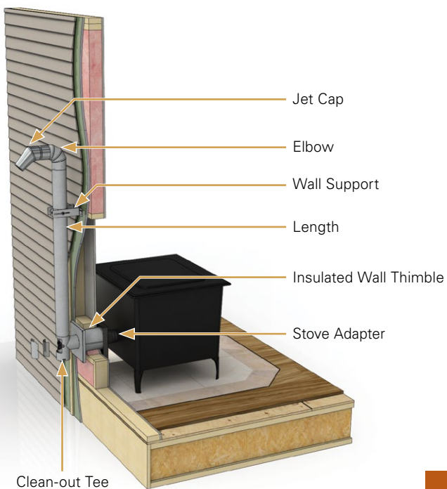
OUT AND UP installation with clean-out tee and jet cap
