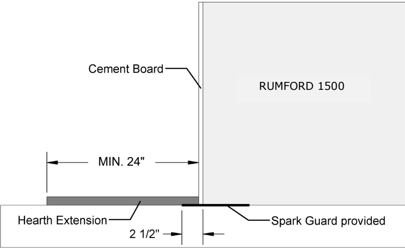
FIGURE 11 STANDARD HEARTH EXTENSION
