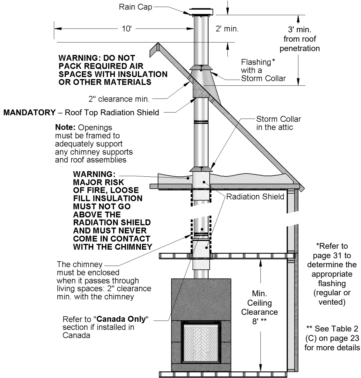
FIGURE 4 GENERAL CHIMNEY REQUIREMENTS
