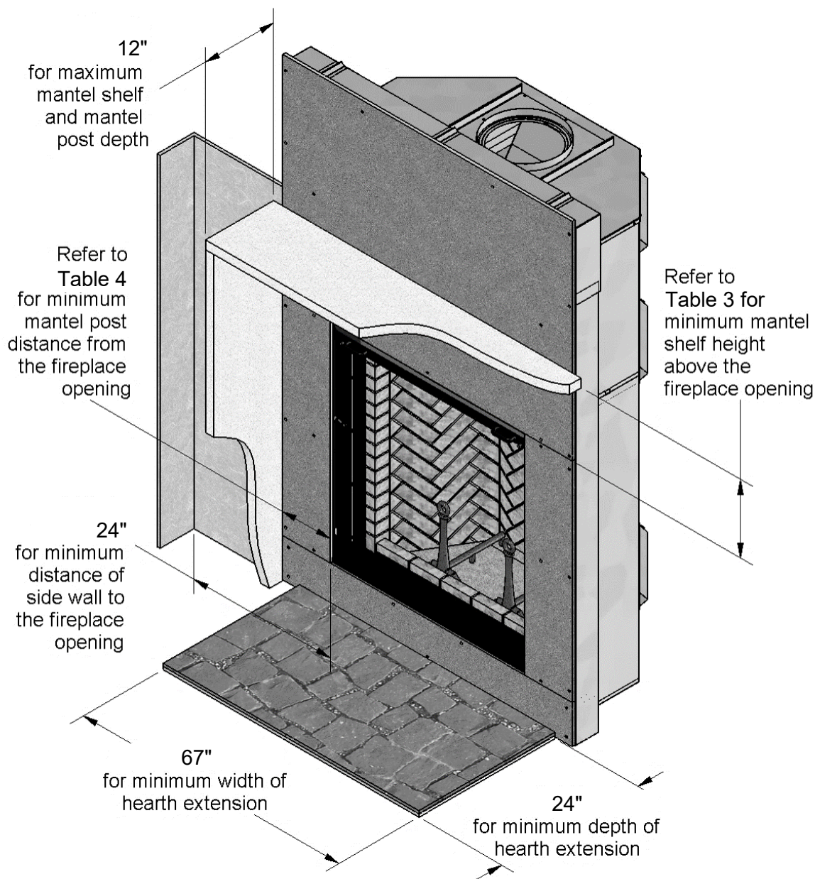
FIGURE 10 FIREPLACE CLEARANCES (SEE TABLE 2)
