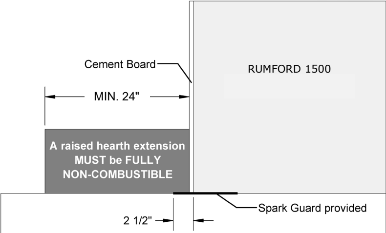
FIGURE 13 RAISED HEARTH EXTENSION
