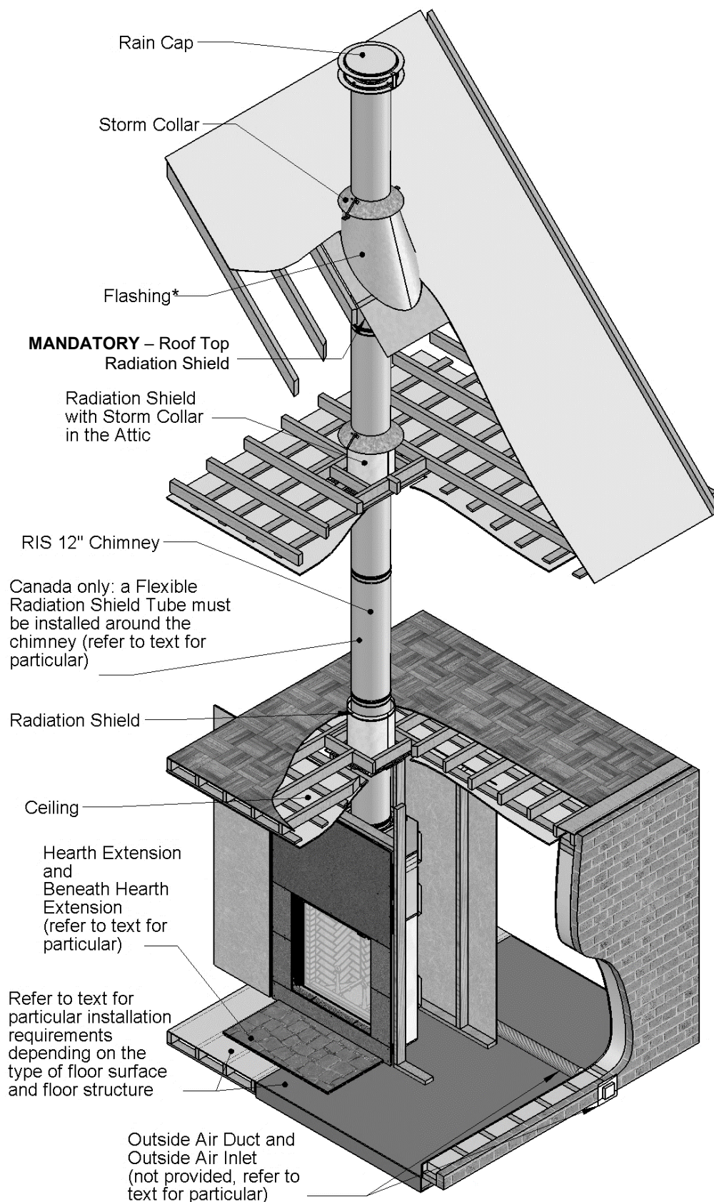
FIGURE 1 GENERAL INSTALLATION OVERVIEW
