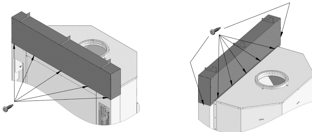
FIGURE 6 INSTALLATION OF THE TOP FINISHING COVER
