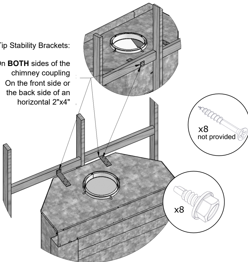
FIGURE 9 ANTI-TIP BRACKET INSTALLATION
