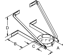
Support mural prolongé (EWSE)
