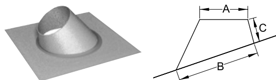
Solin ajustable (EFA, EFB, EFC)
