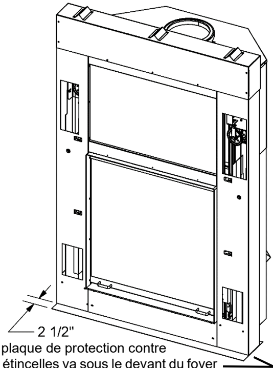
FIGURE 6 SPARK GUARD INSTALLATION
